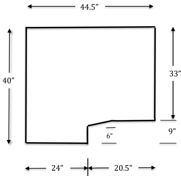
K9 Compartment floor Top View Diagram
